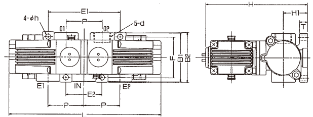
BN-7M47-10A~40A
