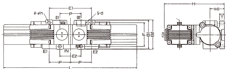
BN-7M47C-10A~40A
