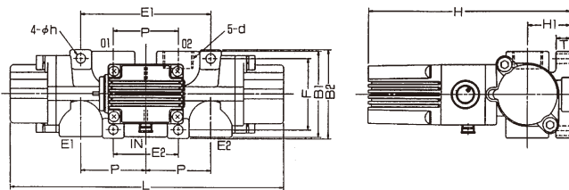
BN-7M43-10A~40A
